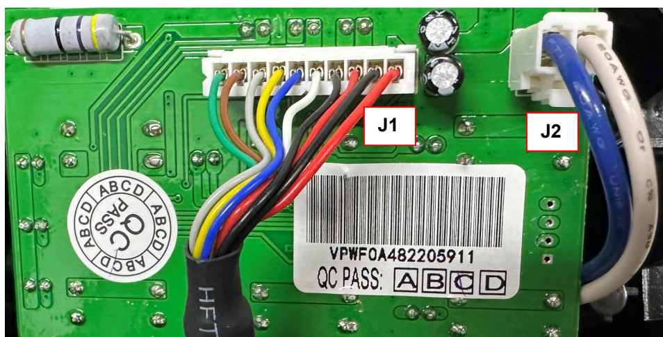
Figure 1. Connectors on Dashboard (EB1)
